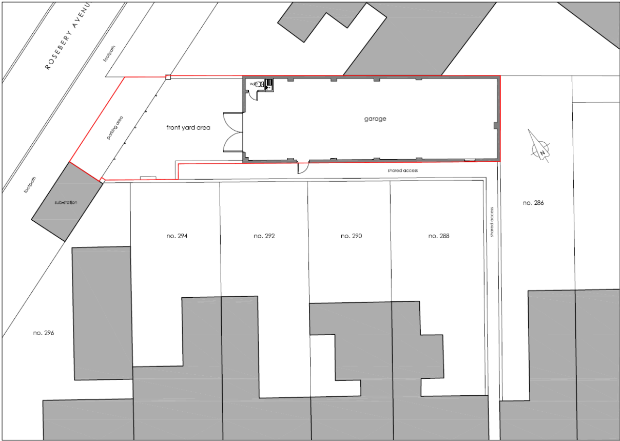
Existing Site
